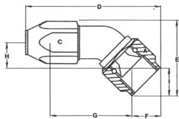
45° Non-Adjustable Low Profile Speed Seal Hose End
