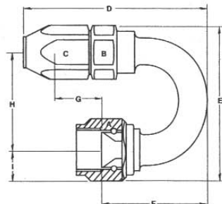
180° Tubular Swivel Seal
