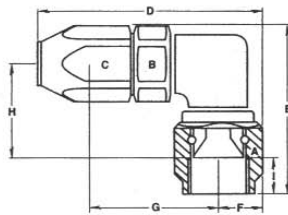
90° Low Profile Swivel Seal Hose End
