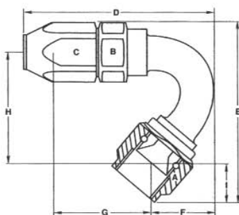
120° Tubular Auto-Fit Hose End
