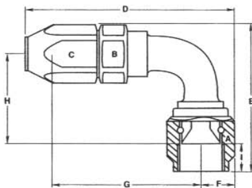
90° Tubular Auto-Fit Hose End
