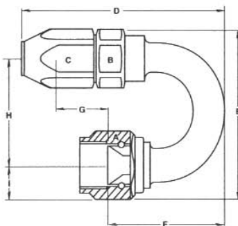
180° Tubular Auto-Fit Hose End
