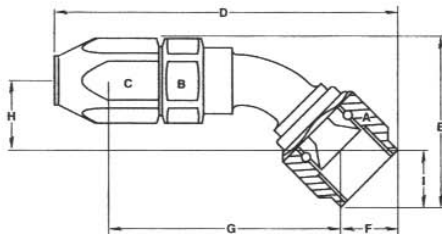
45° Tubular Auto-Fit Hose End
