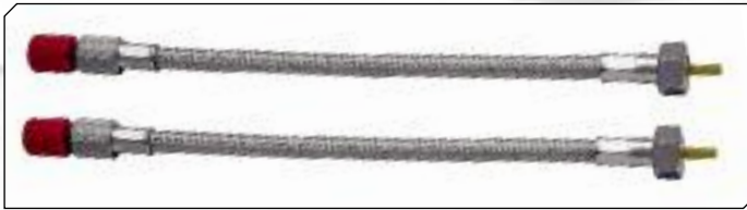
D-Spec/HTS Adjustment Extensions TO00100 Flexible 8" extension features Braided Stainless Steel cover, knurled and anodized adjuster knob with etched markings. Great for hard to reach rear shocks like G-35, 350Z, Mustang and others. Sold in pairs.
