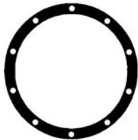
8-3/8" X 9-3/32" 10 HOLE ROUND
