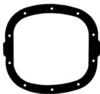
8-5/16" X 10-9/16" 10 HOLES OVAL
